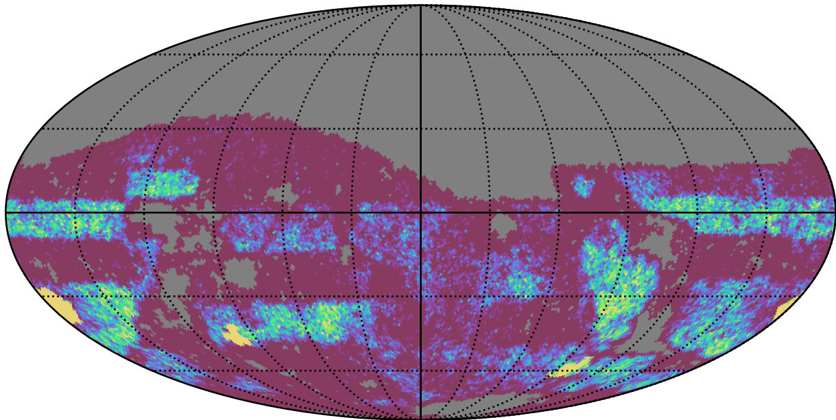
too_elab_r16_d3_griz_v3.4_10yrs Yr 3-4 g band: NVisits
