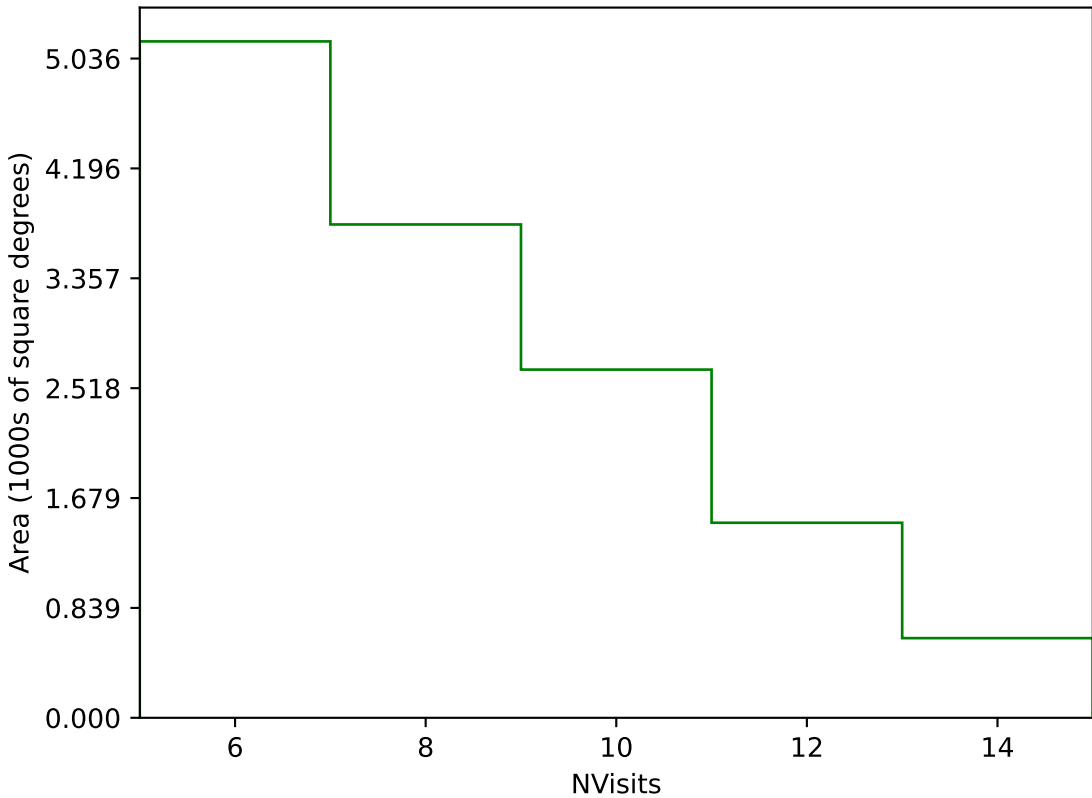
too_elab_r16_d3_griz_v3.4_10yrs Yr 3-4 g band: NVisits
