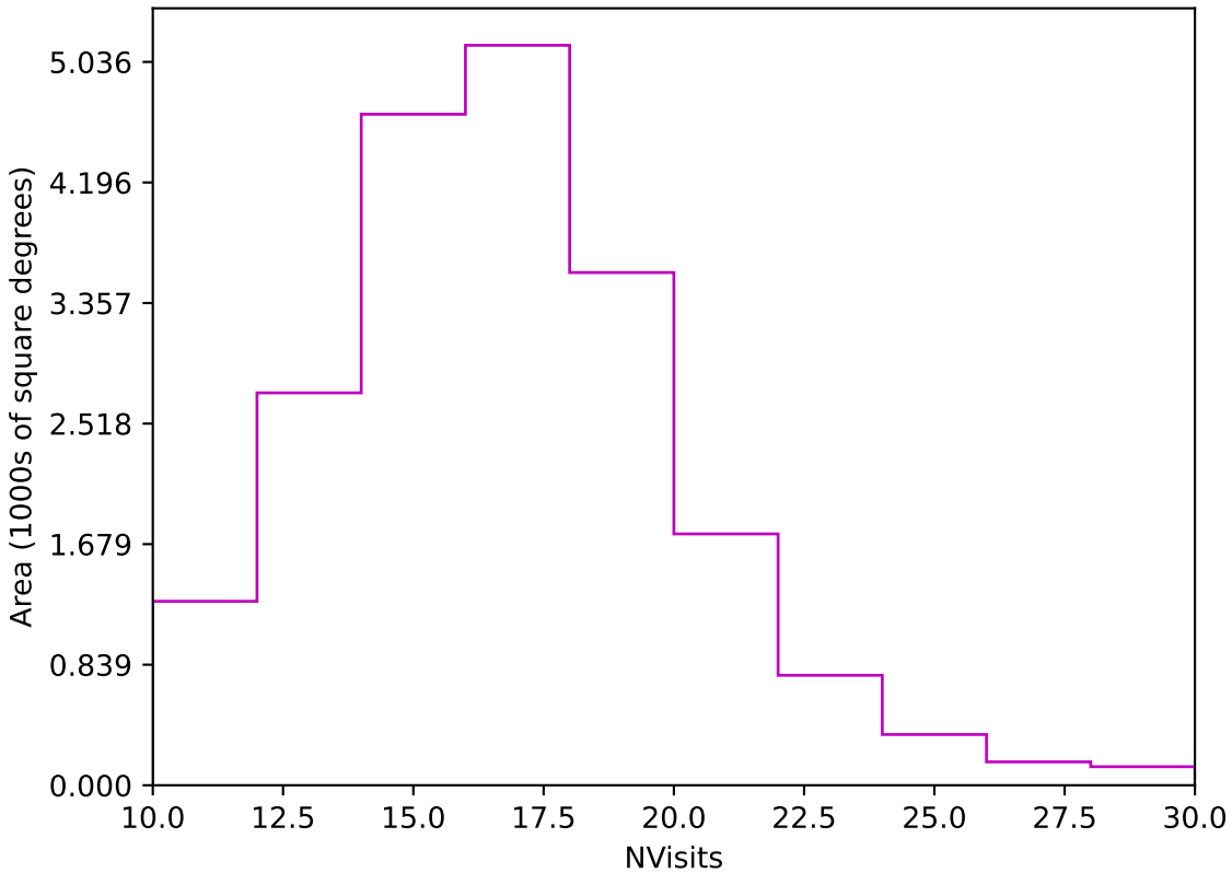
too_elab_r16_d3_griz_v3.4_10yrs Yr 1 z band: NVisits
