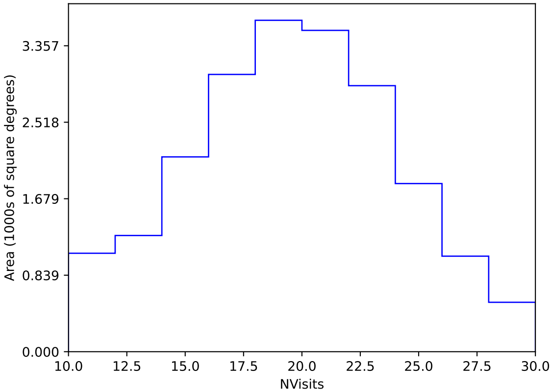
too_elab_r16_d3_griz_v3.4_10yrs Yr 1 y band: NVisits
