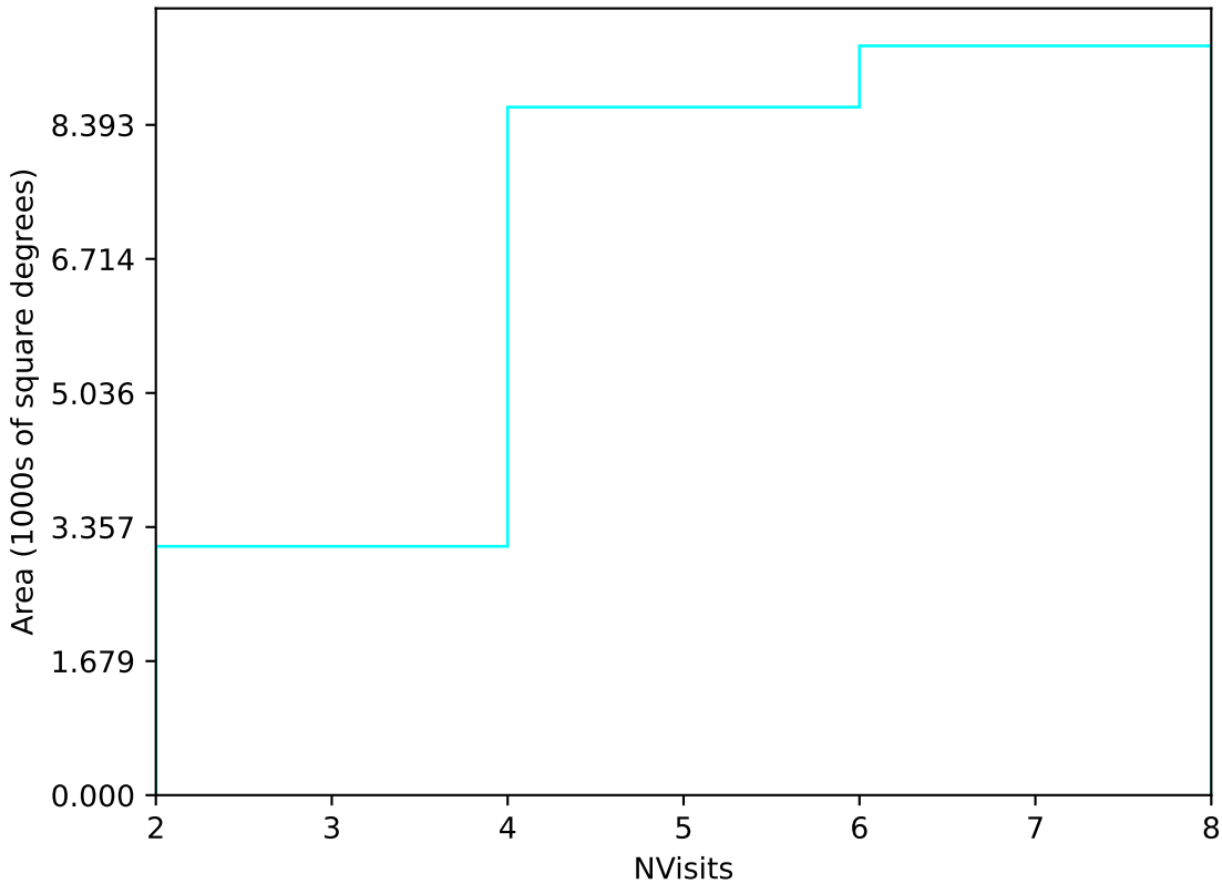
too_elab_r16_d3_griz_v3.4_10yrs Yr 1 u band: NVisits
