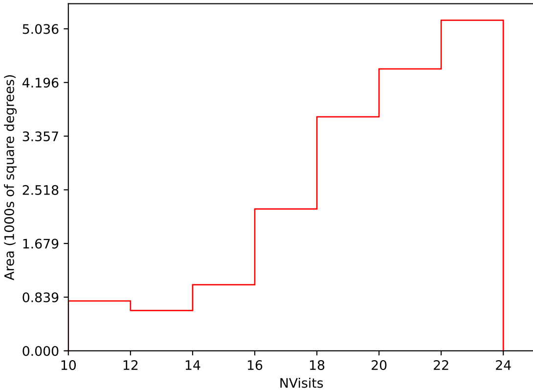
too_elab_r16_d3_griz_v3.4_10yrs Yr 1 i band: NVisits
