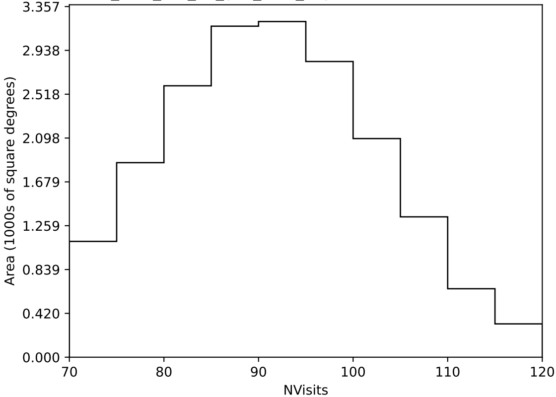
too_elab_r16_d3_griz_v3.4_10yrs Yr 1 all bands: NVisits
