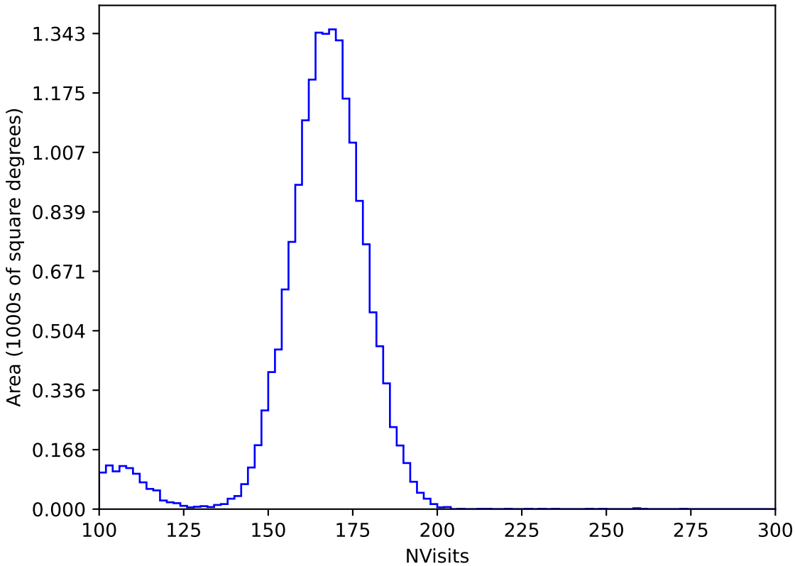
too_elab_r16_d3_griz_v3.4_10yrs WFD y band: NVisits
