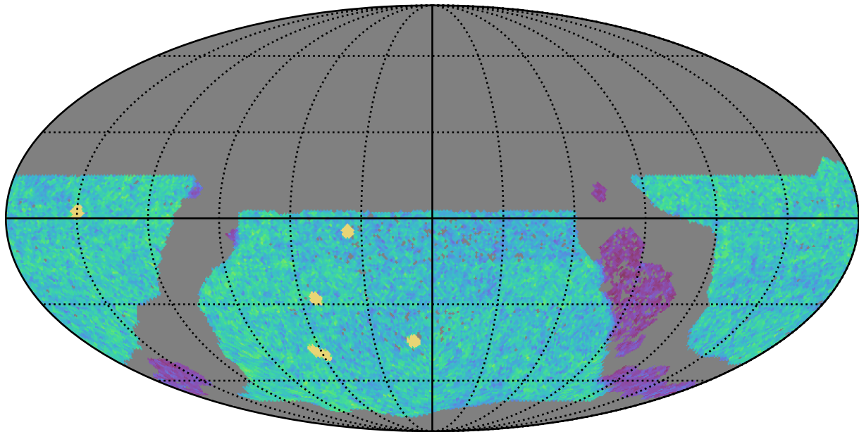
too_elab_r16_d3_griz_v3.4_10yrs WFD u band: NVisits
