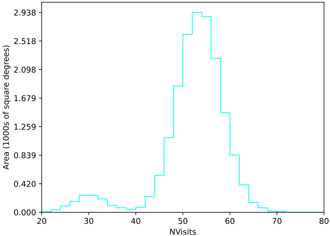
too_elab_r16_d3_griz_v3.4_10yrs WFD u band: NVisits
