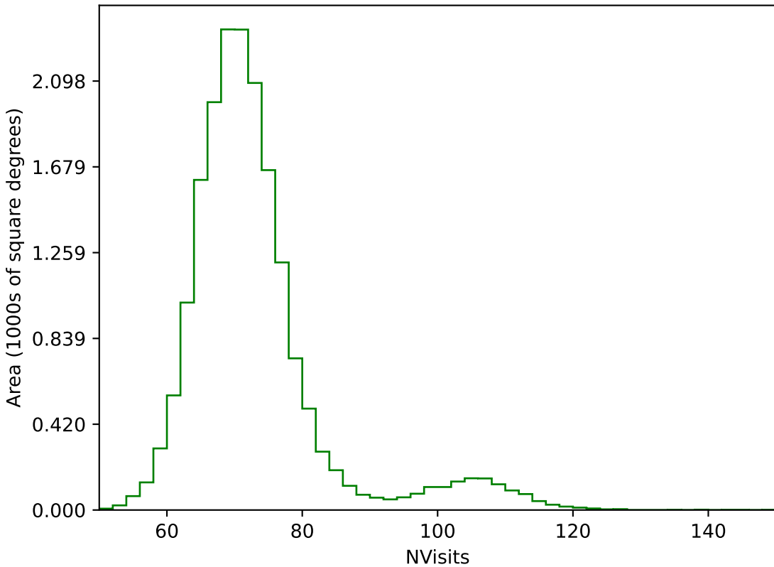
too_elab_r16_d3_griz_v3.4_10yrs WFD g band: NVisits
