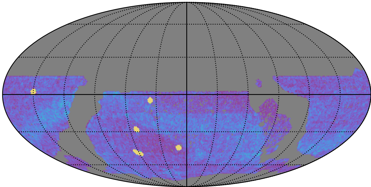
too_elab_r16_d3_griz_v3.4_10yrs WFD all bands: NVisits
