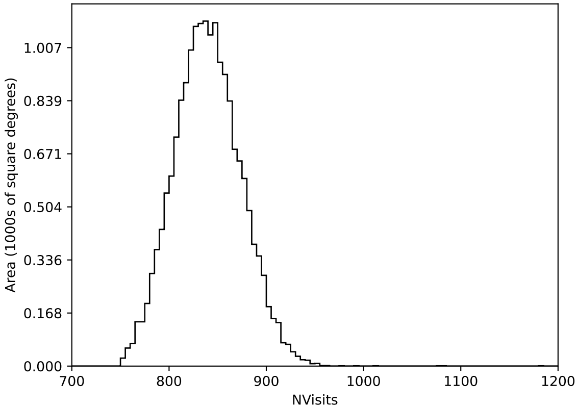
too_elab_r16_d3_griz_v3.4_10yrs WFD all bands: NVisits
