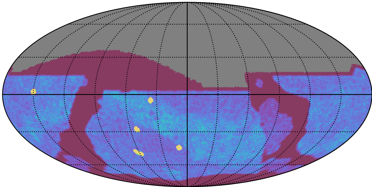
too_elab_r16_d3_griz_v3.4_10yrs All sky z band: NVisits
