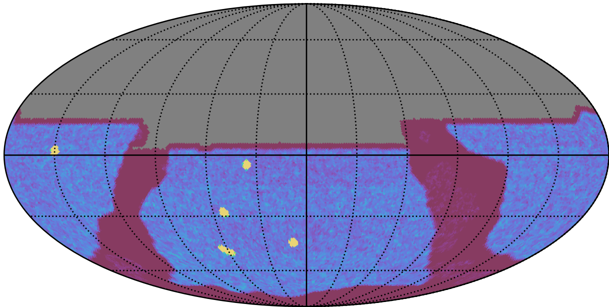
too_elab_r16_d3_griz_v3.4_10yrs All sky y band: NVisits
