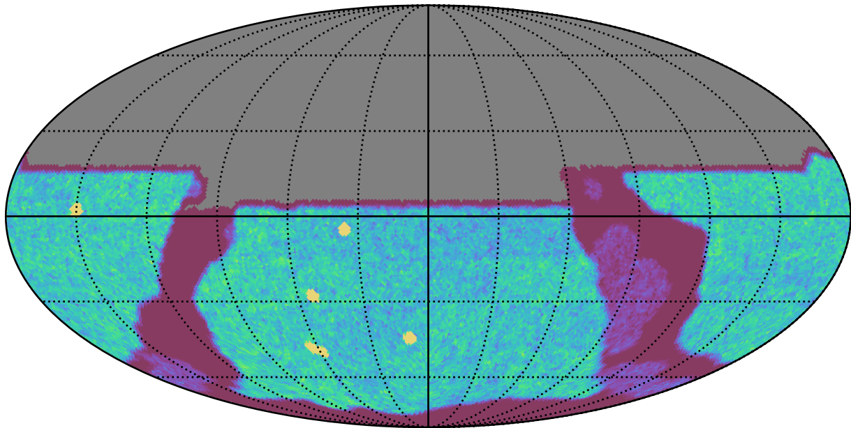
too_elab_r16_d3_griz_v3.4_10yrs All sky u band: NVisits
