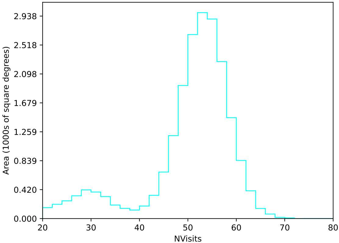
too_elab_r16_d3_griz_v3.4_10yrs All sky u band: NVisits
