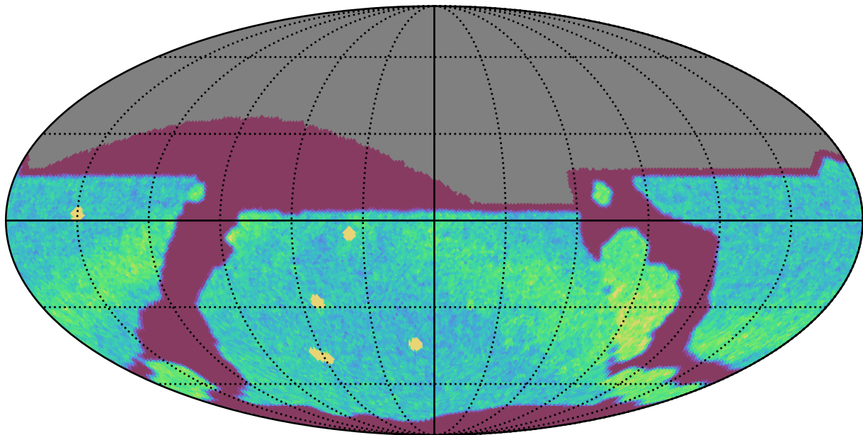
too_elab_r16_d3_griz_v3.4_10yrs All sky r band: NVisits
