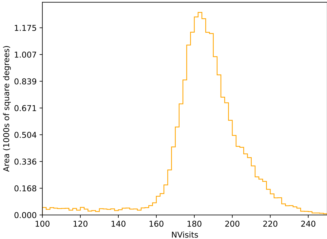
too_elab_r16_d3_griz_v3.4_10yrs All sky r band: NVisits
