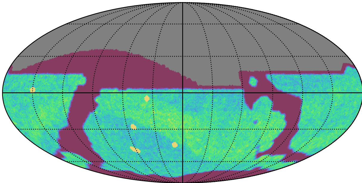
too_elab_r16_d3_griz_v3.4_10yrs All sky i band: NVisits
