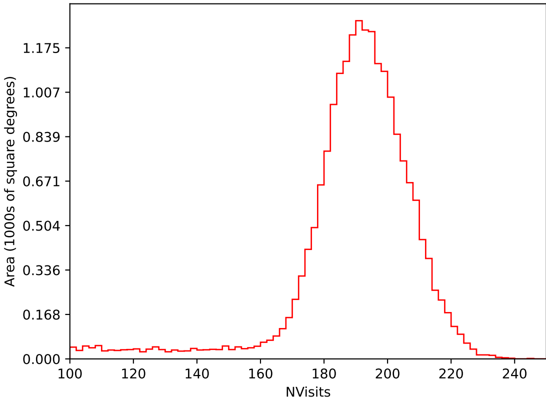
too_elab_r16_d3_griz_v3.4_10yrs All sky i band: NVisits
