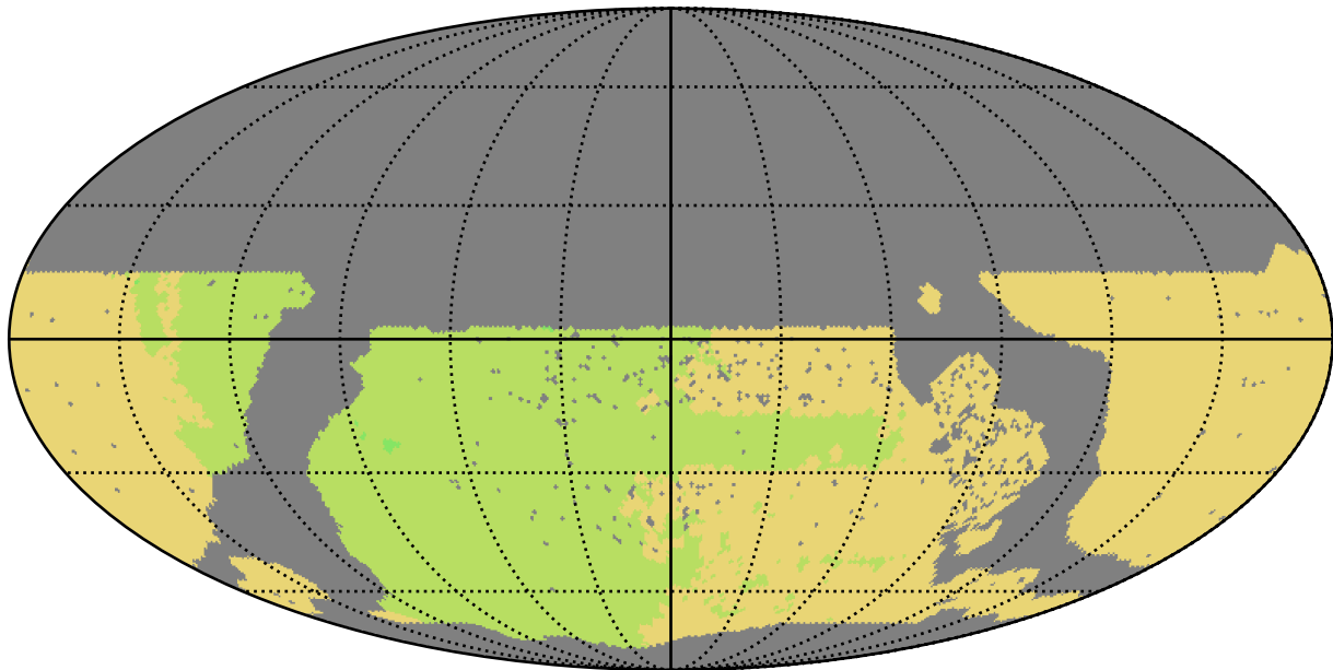
too_elab_r16_d3_griz_v3.4_10yrs WFD all bands: NSeasons
