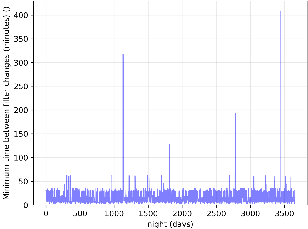
too_elab_r16_d3_griz_v3.4_10yrs Per Night: Minimum time between filter changes (minutes)
