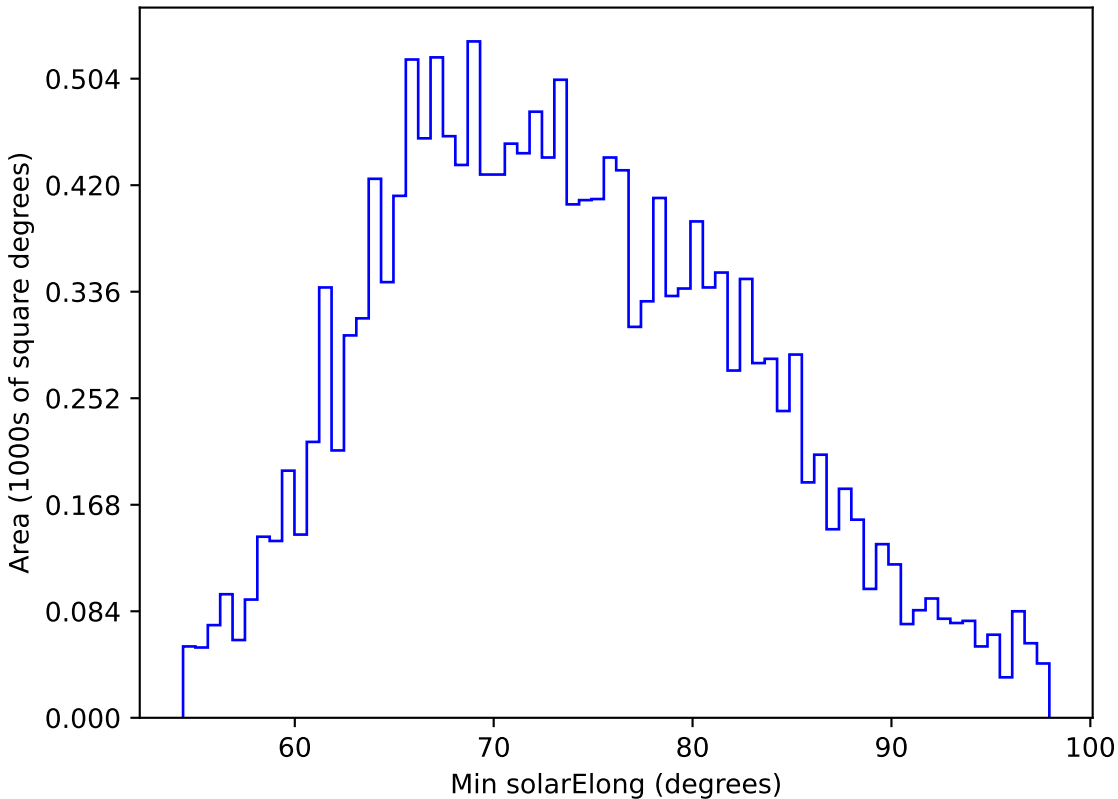
too_elab_r16_d3_griz_v3.4_10yrs WFD g band: Min solarElong
