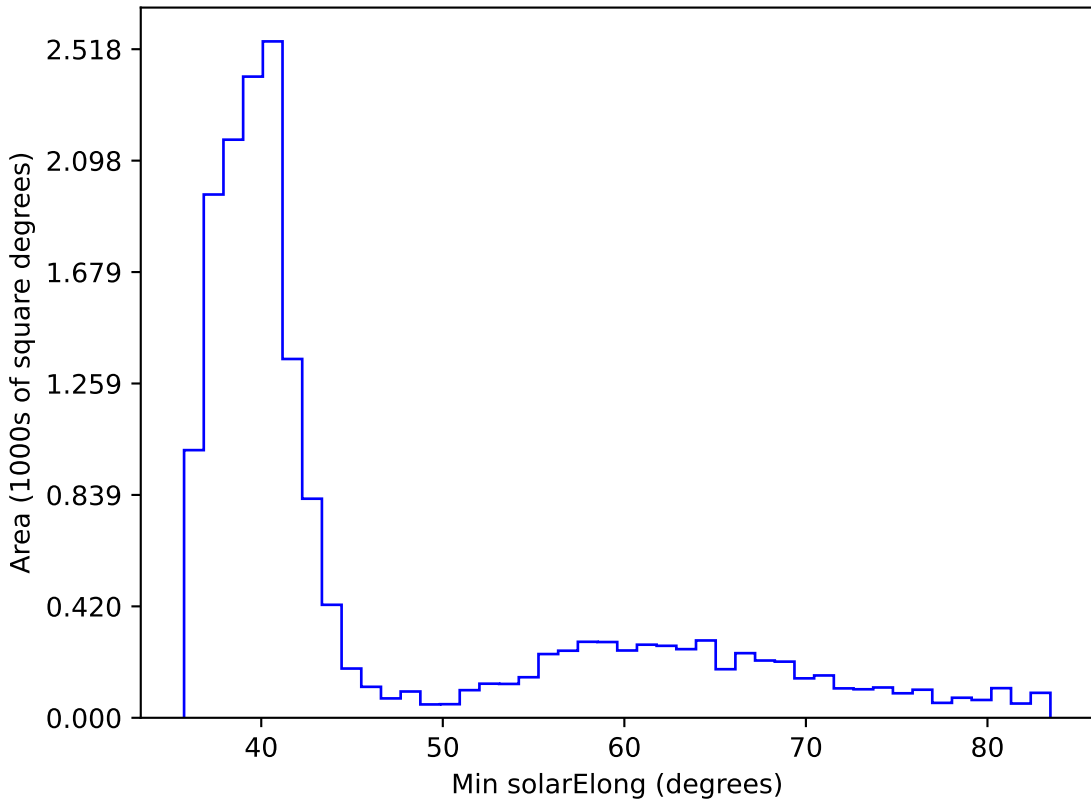
too_elab_r16_d3_griz_v3.4_10yrs WFD all bands: Min solarElong
