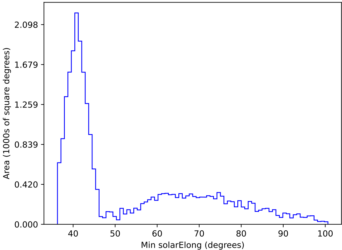
too_elab_r16_d3_griz_v3.4_10yrs All sky z band: Min solarElong
