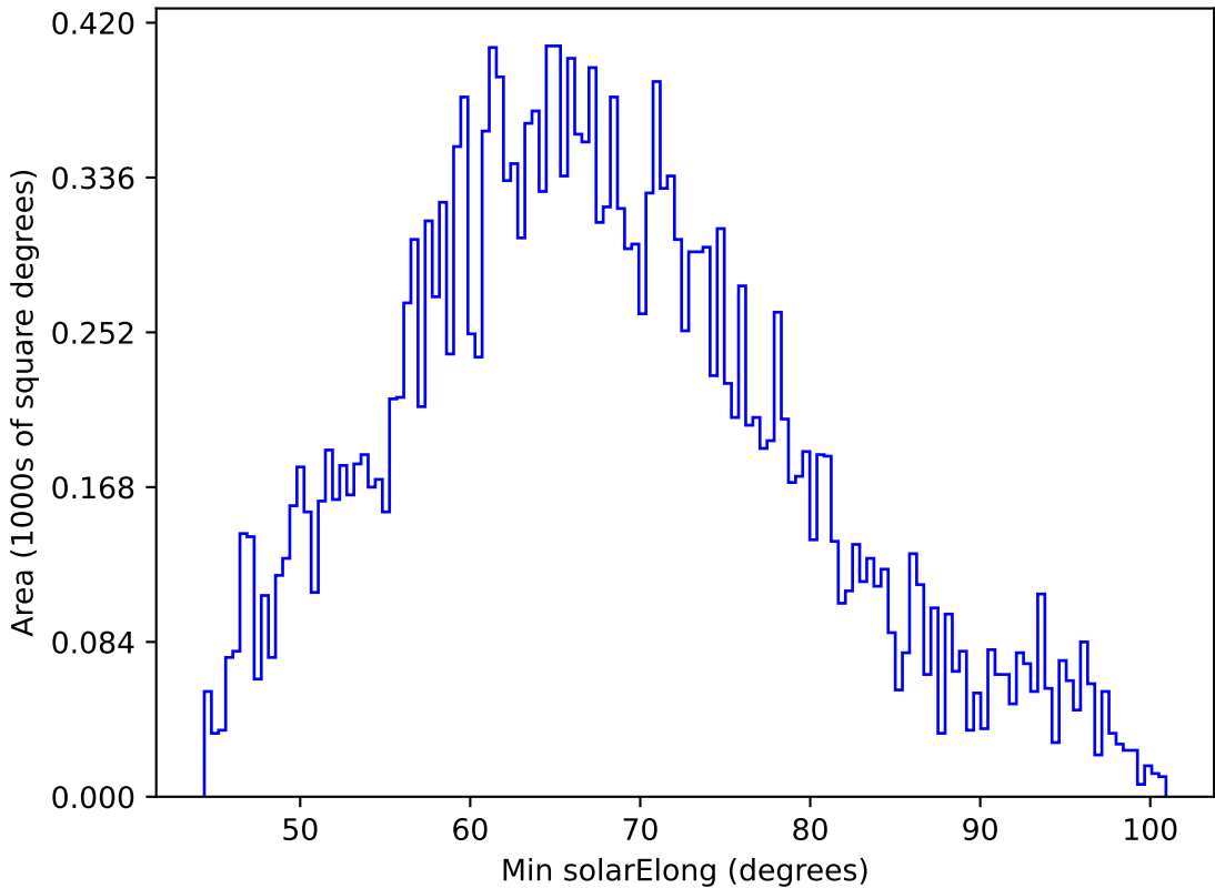
too_elab_r16_d3_griz_v3.4_10yrs All sky y band: Min solarElong
