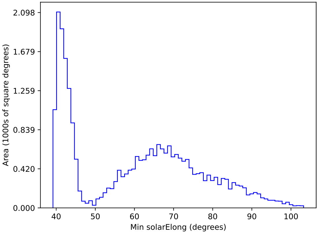
too_elab_r16_d3_griz_v3.4_10yrs All sky r band: Min solarElong
