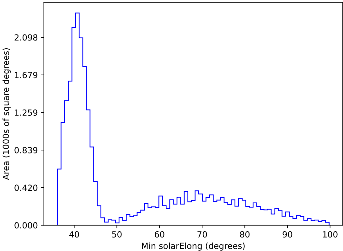
too_elab_r16_d3_griz_v3.4_10yrs All sky i band: Min solarElong
