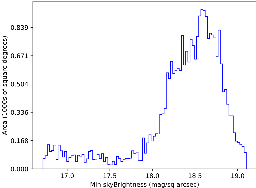
too_elab_r16_d3_griz_v3.4_10yrs Yr 1 z band: Min skyBrightness
