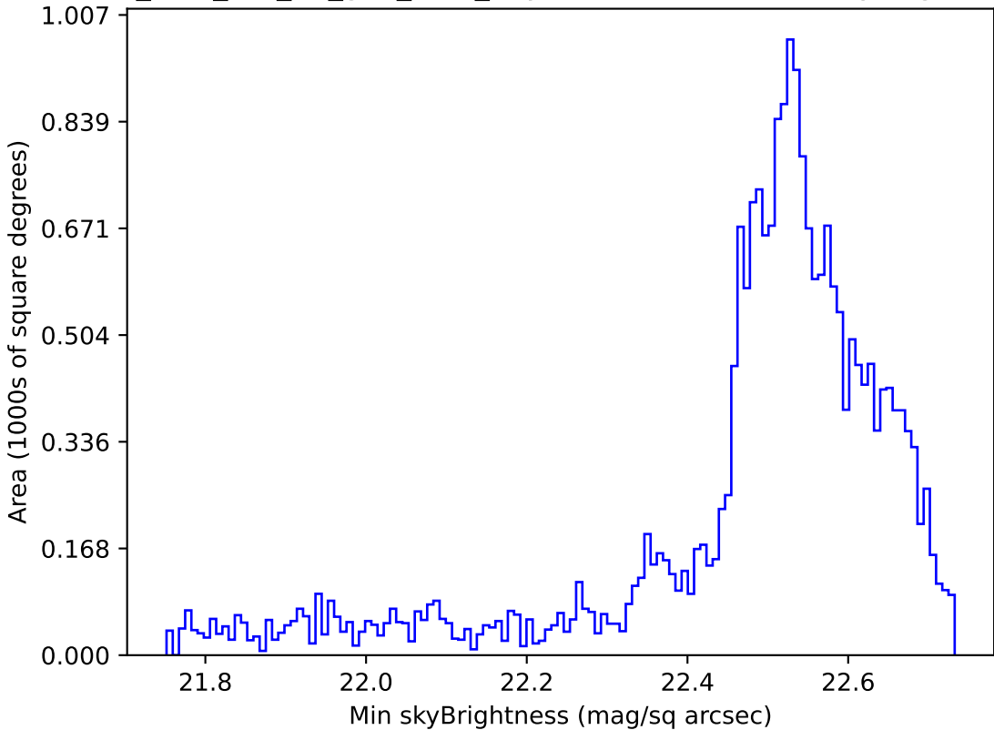
too_elab_r16_d3_griz_v3.4_10yrs Yr 1 u band: Min skyBrightness
