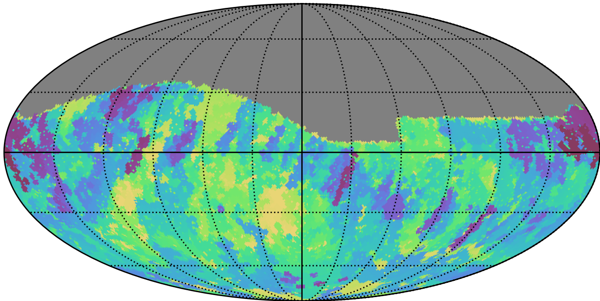
too_elab_r16_d3_griz_v3.4_10yrs Yr 1 r band: Min skyBrightness
