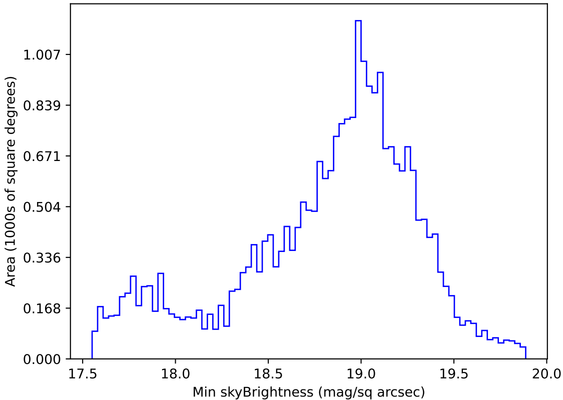
too_elab_r16_d3_griz_v3.4_10yrs Yr 1 i band: Min skyBrightness
