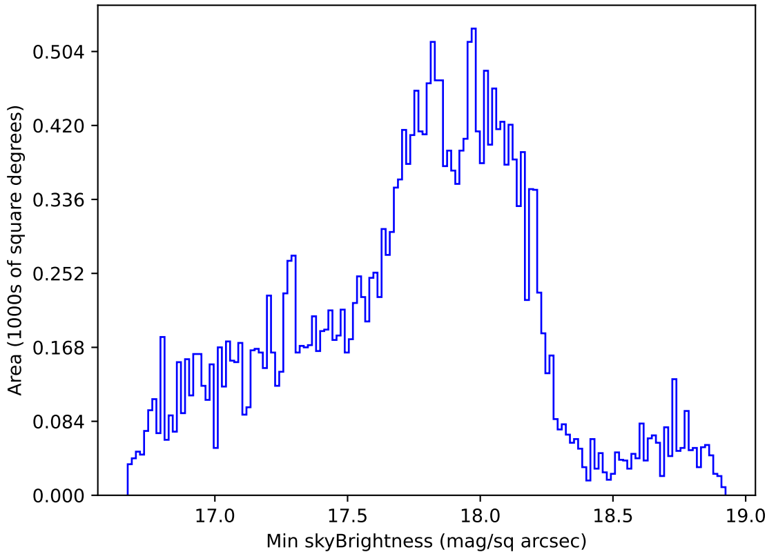
too_elab_r16_d3_griz_v3.4_10yrs Yr 1 all bands: Min skyBrightness
