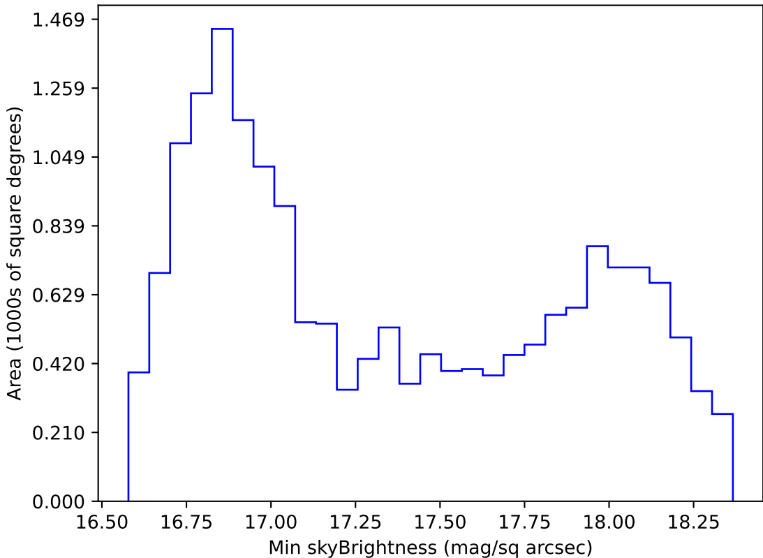
too_elab_r16_d3_griz_v3.4_10yrs WFD z band: Min skyBrightness
