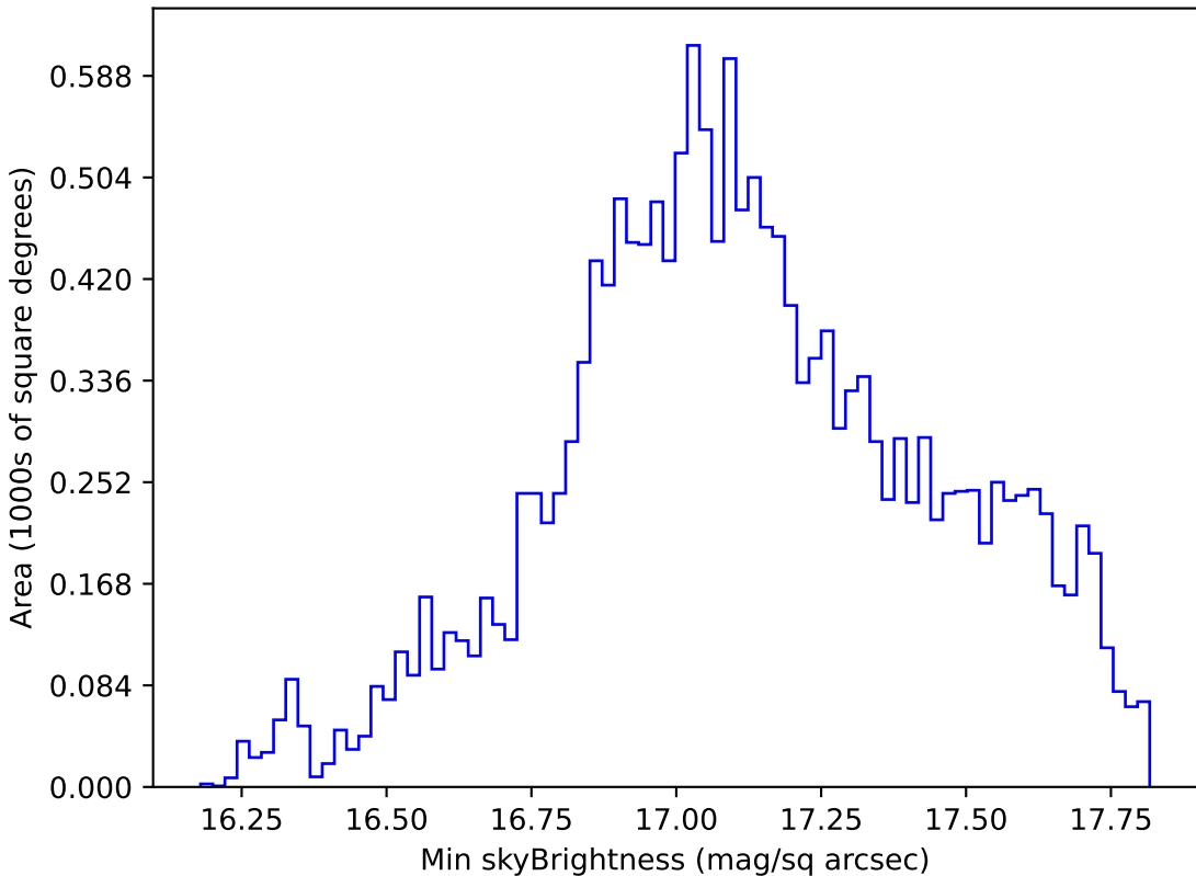
too_elab_r16_d3_griz_v3.4_10yrs WFD y band: Min skyBrightness
