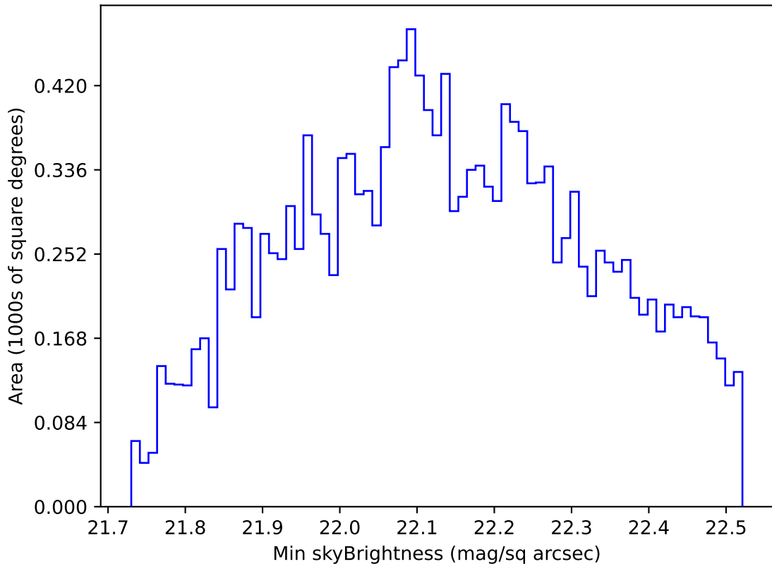
too_elab_r16_d3_griz_v3.4_10yrs WFD u band: Min skyBrightness
