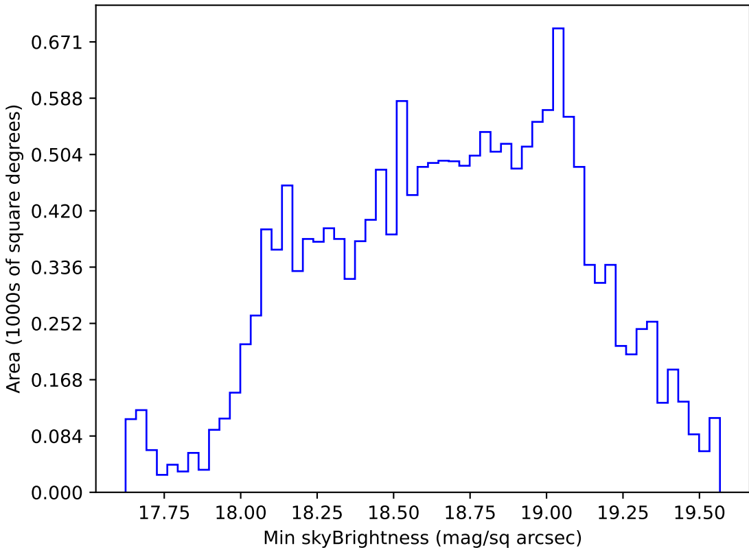
too_elab_r16_d3_griz_v3.4_10yrs WFD r band: Min skyBrightness
