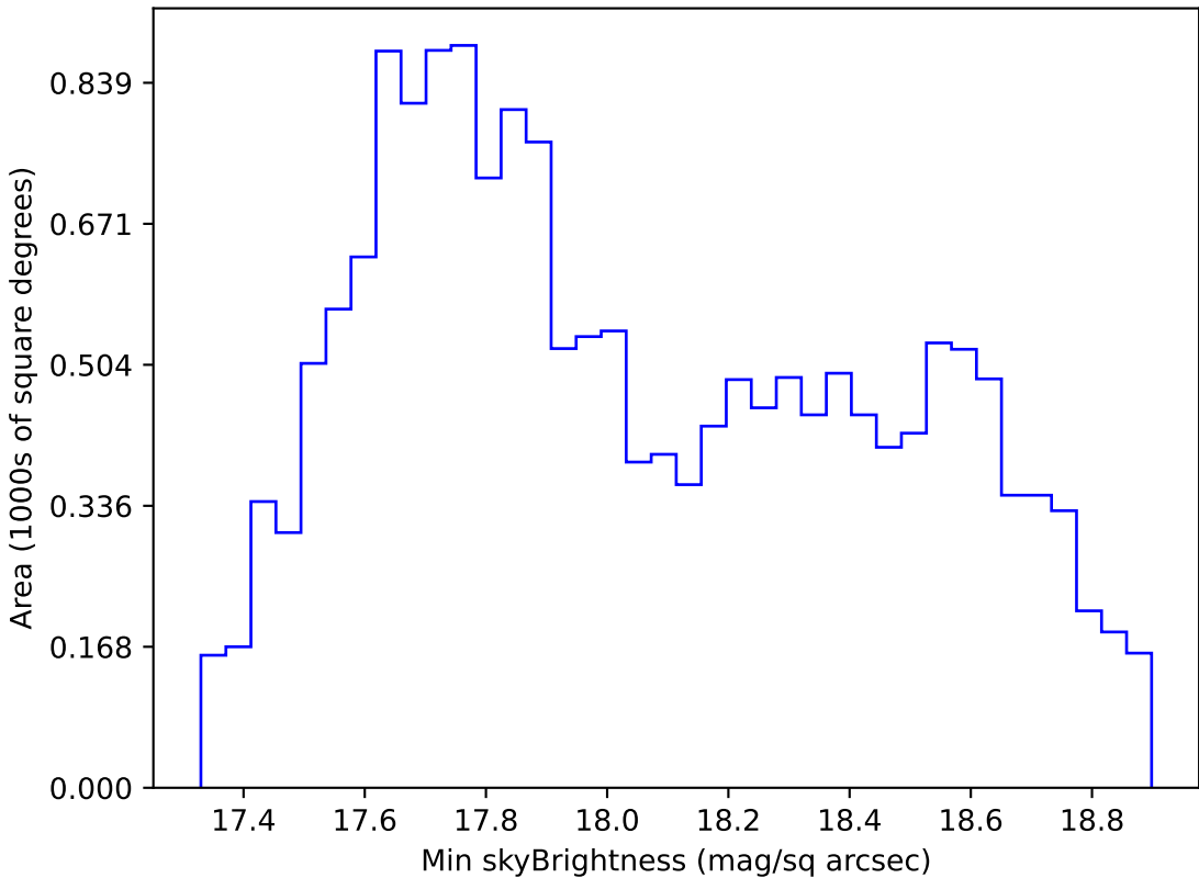
too_elab_r16_d3_griz_v3.4_10yrs WFD i band: Min skyBrightness
