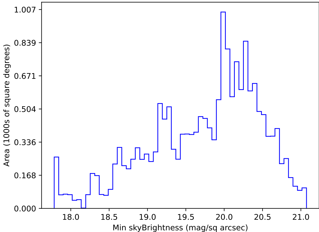
too_elab_r16_d3_griz_v3.4_10yrs WFD g band: Min skyBrightness
