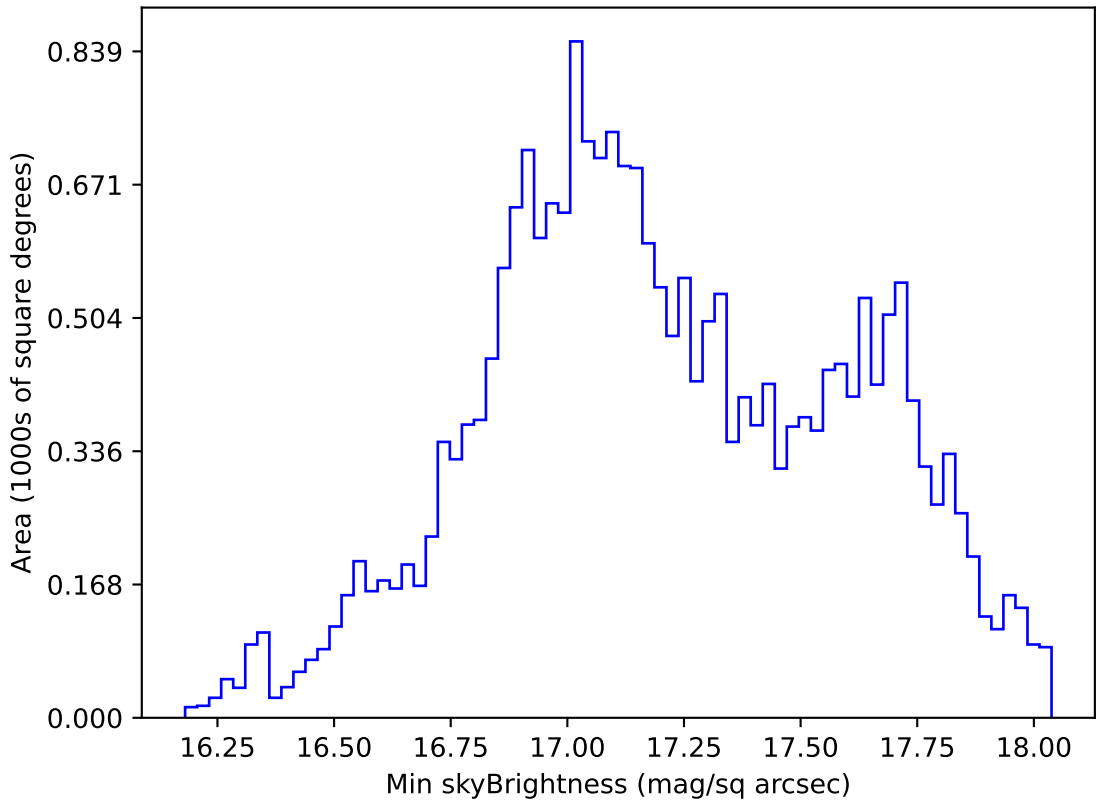
too_elab_r16_d3_griz_v3.4_10yrs All sky y band: Min skyBrightness
