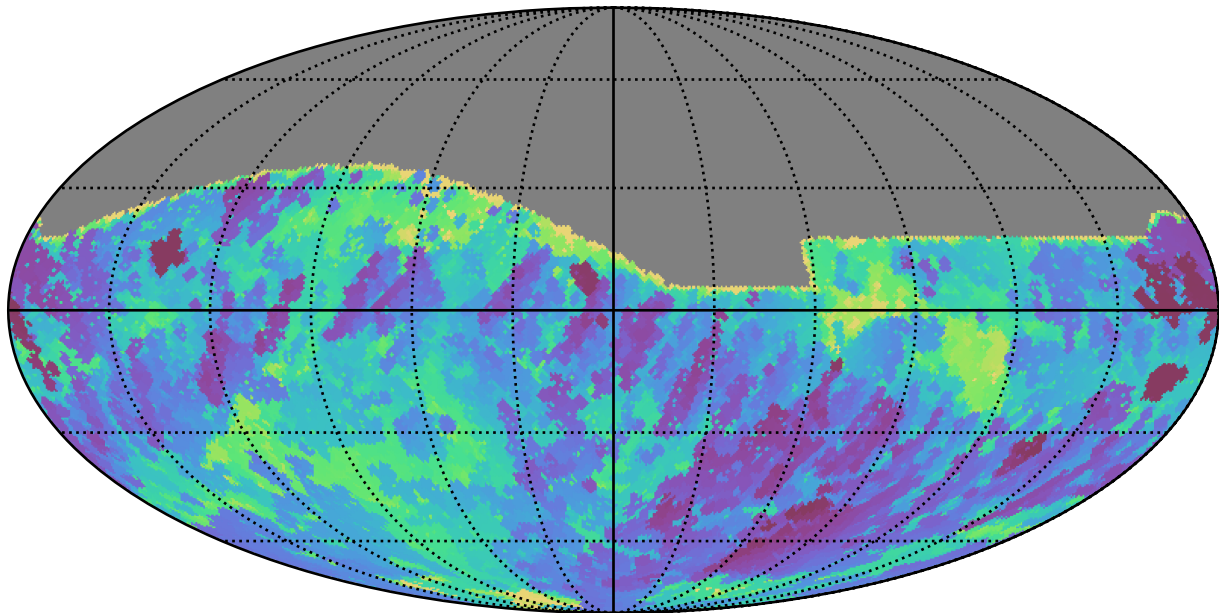
too_elab_r16_d3_griz_v3.4_10yrs All sky r band: Min skyBrightness
