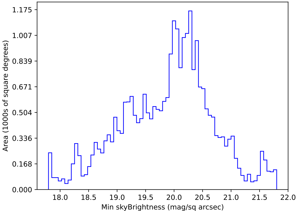
too_elab_r16_d3_griz_v3.4_10yrs All sky g band: Min skyBrightness
