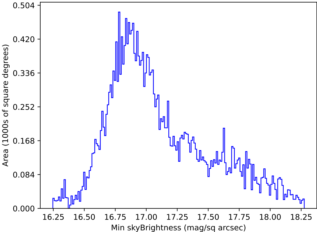
too_elab_r16_d3_griz_v3.4_10yrs All sky all bands: Min skyBrightness
