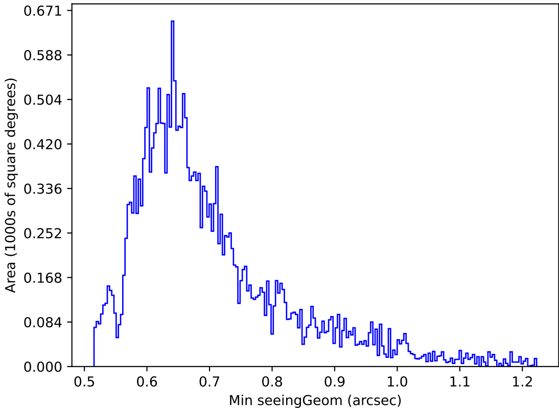
too_elab_r16_d3_griz_v3.4_10yrs Yr 1 g band: Min seeingGeom
