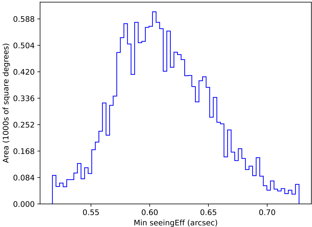
too_elab_r16_d3_griz_v3.4_10yrs WFD z band: Min seeingEff
