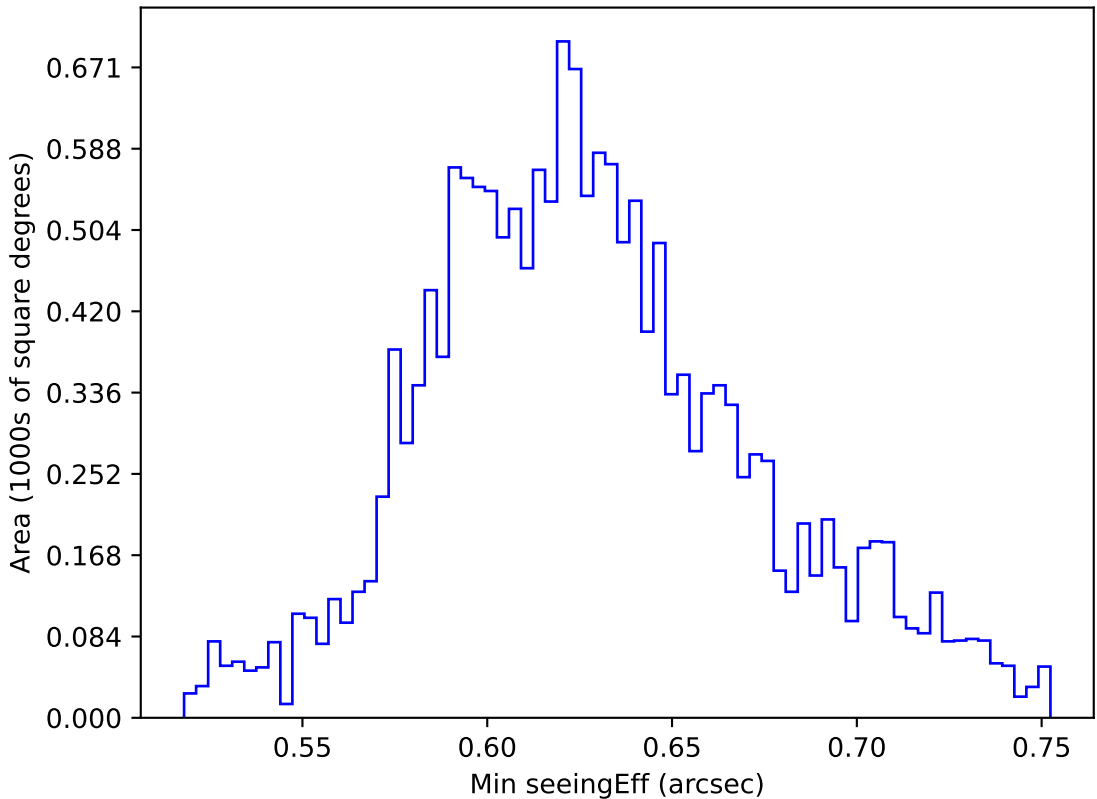
too_elab_r16_d3_griz_v3.4_10yrs WFD y band: Min seeingEff
