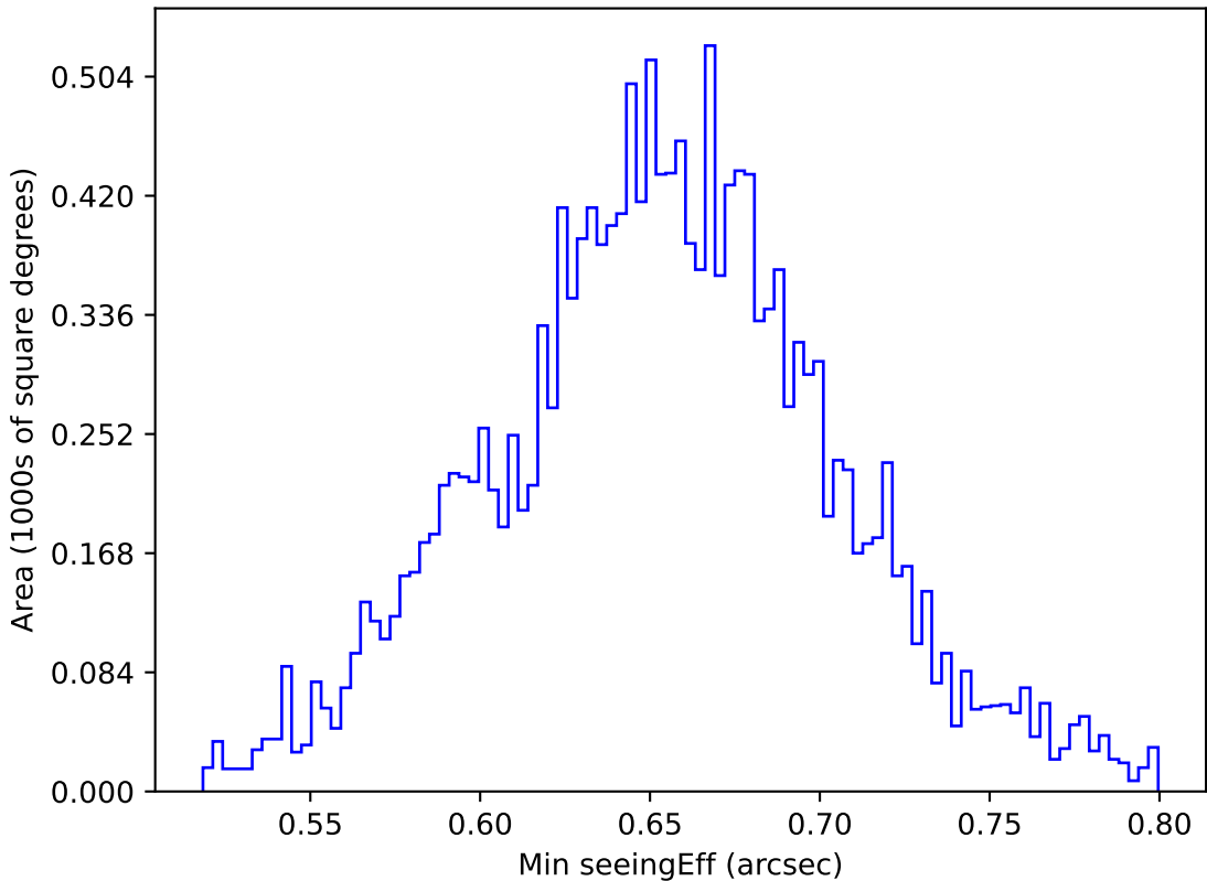
too_elab_r16_d3_griz_v3.4_10yrs WFD g band: Min seeingEff
