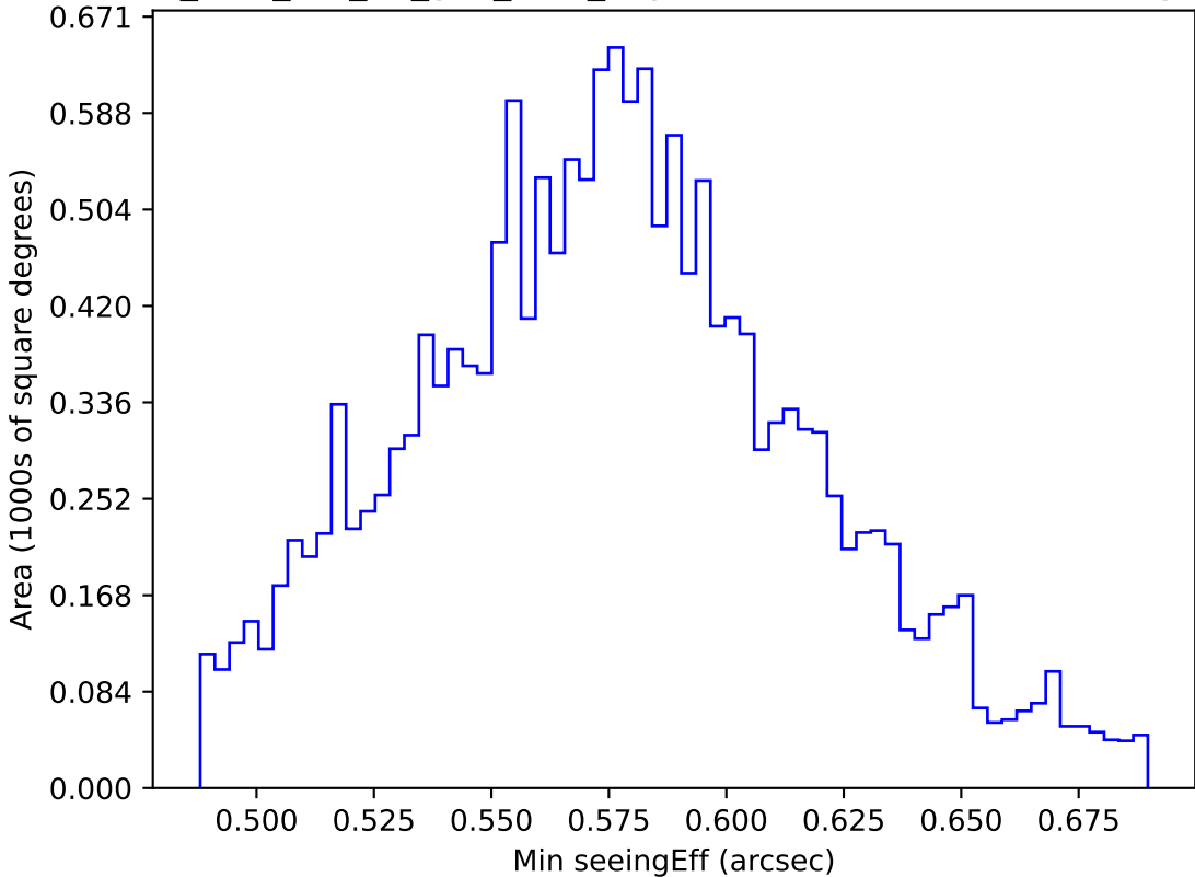
too_elab_r16_d3_griz_v3.4_10yrs WFD all bands: Min seeingEff
