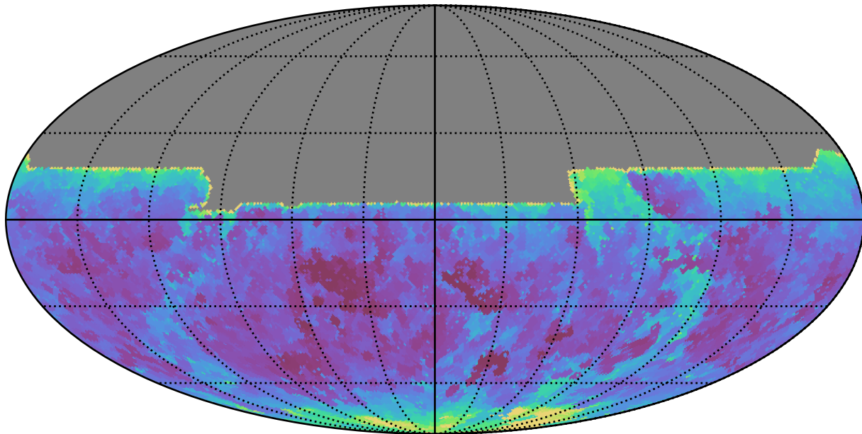
too_elab_r16_d3_griz_v3.4_10yrs All sky y band: Min seeingEff
